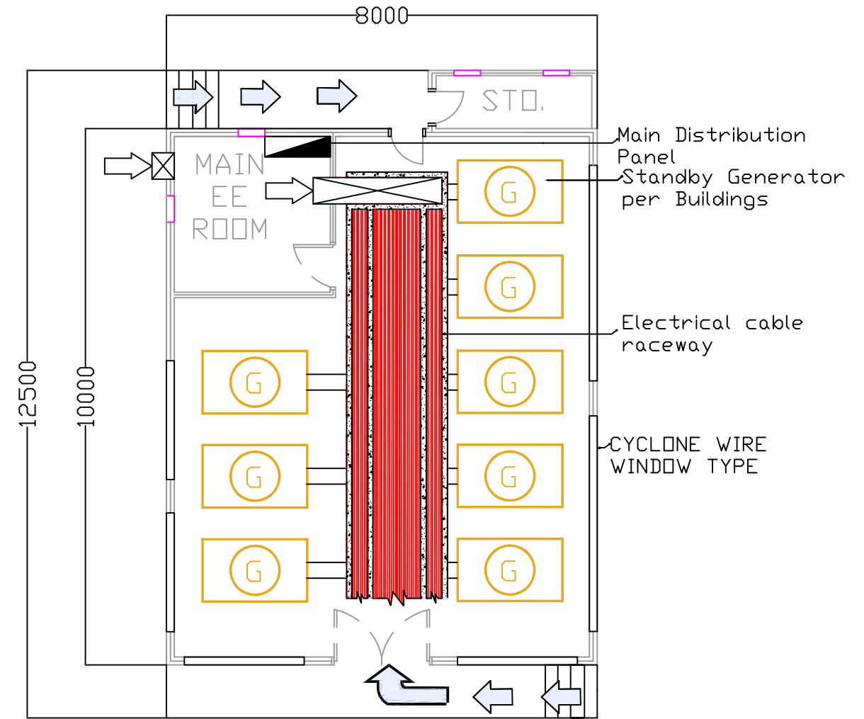
FLOOR PLAN
